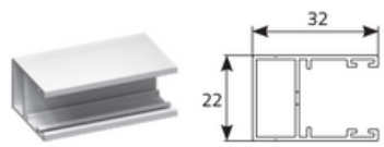
Straight guide
