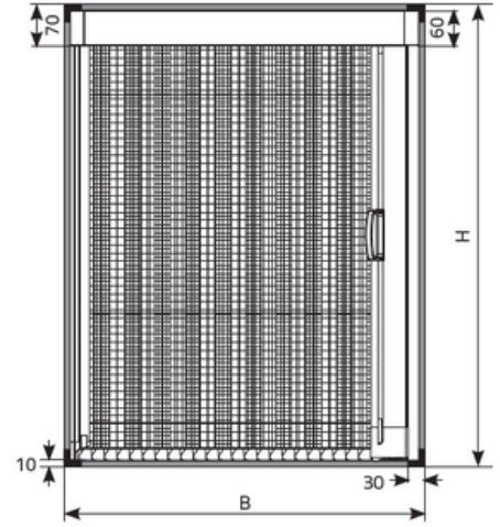
Pleated insect screen with full frame, option 2 (surcharge)
