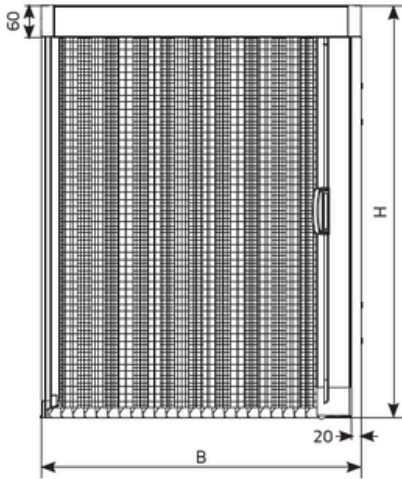
Pleated insect screen without frame
