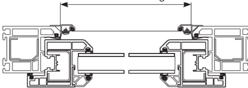
Faced window
