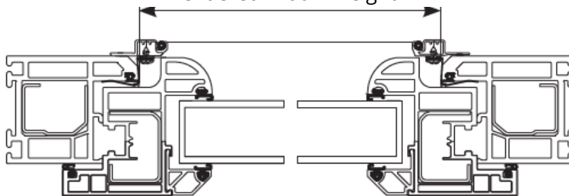
Faced window
