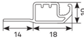
Recessed window
